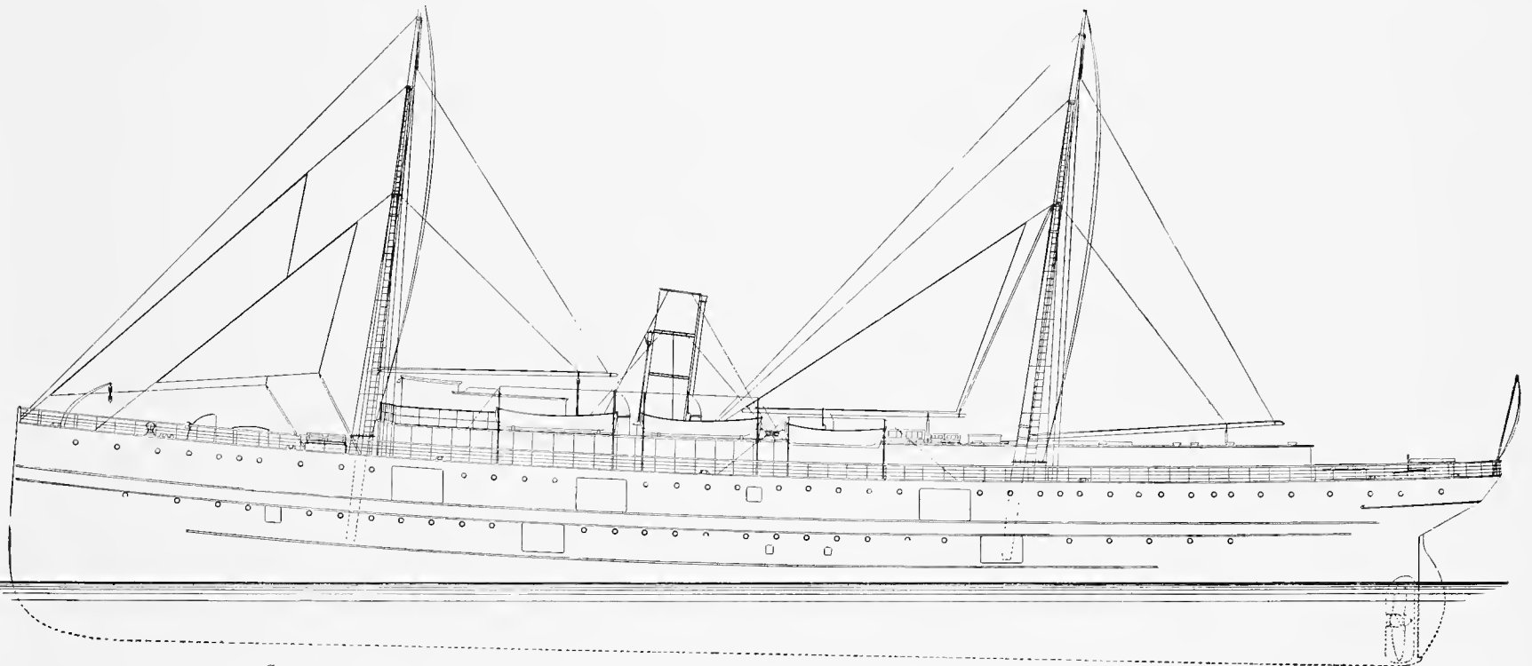
SHEAR PLAN OF THE STEAMSHIP HOWARD, OF THE MERCHANTS' AND MINERS' LINE, BALTIMORE, MD.
